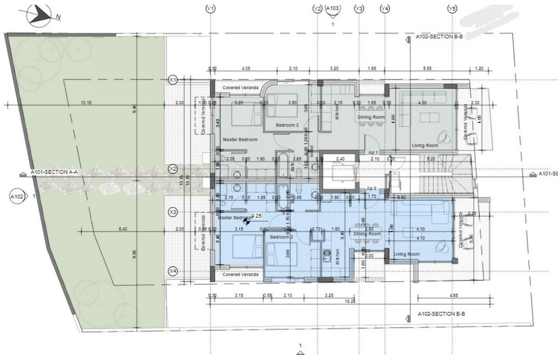
First Floor Plan B-B
