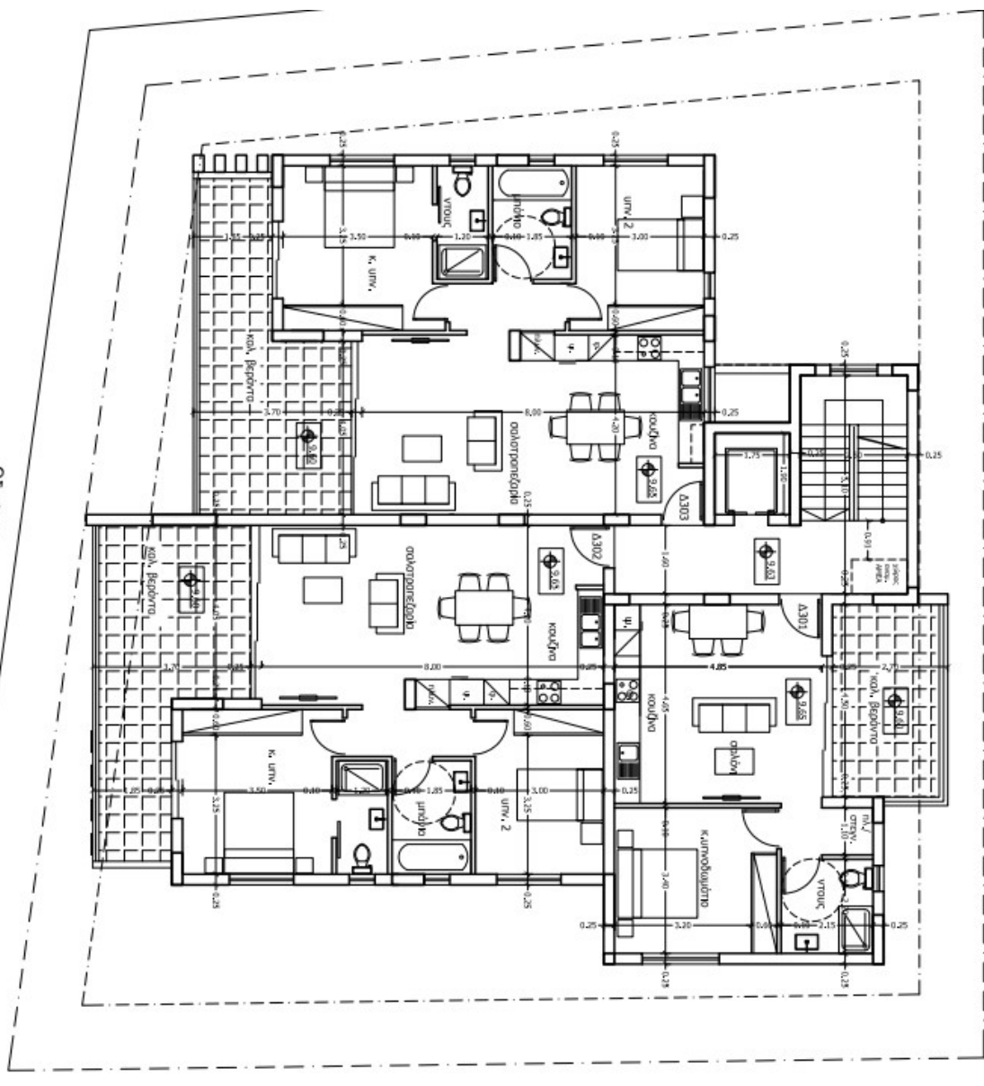
Third Floor Plan .jpg
