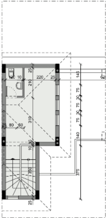
ATTIC FLOOR PLAN
