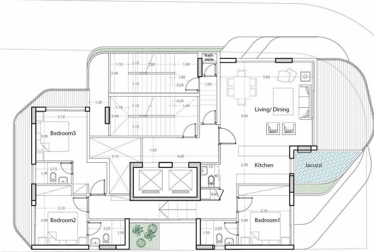
Residence Whole Floor Plan
