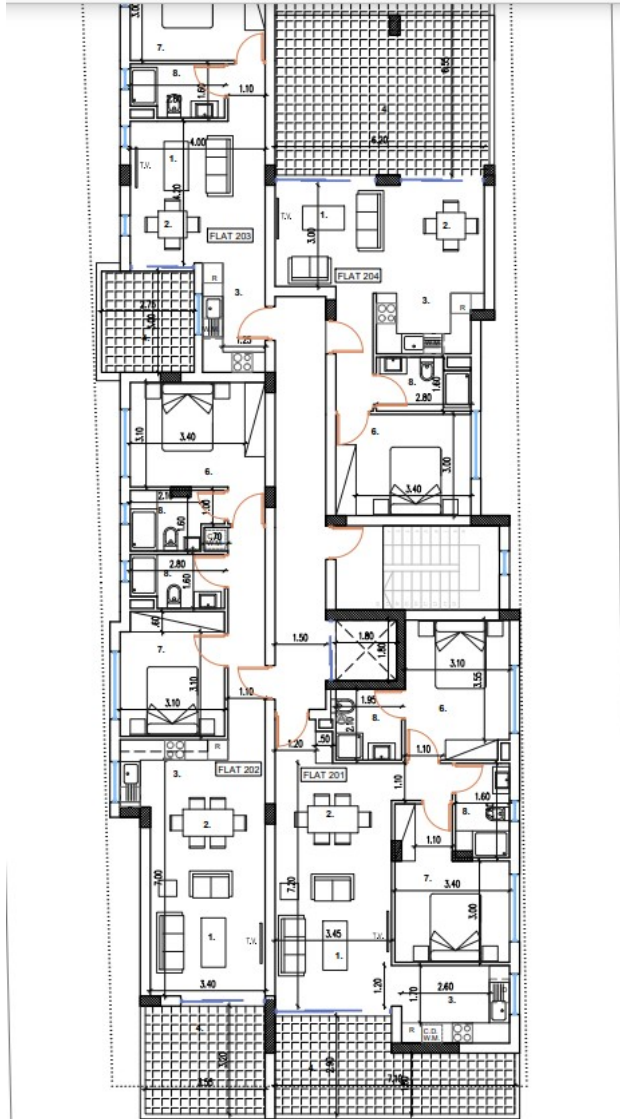
SECOND FLOOR PLAN OPTION A
