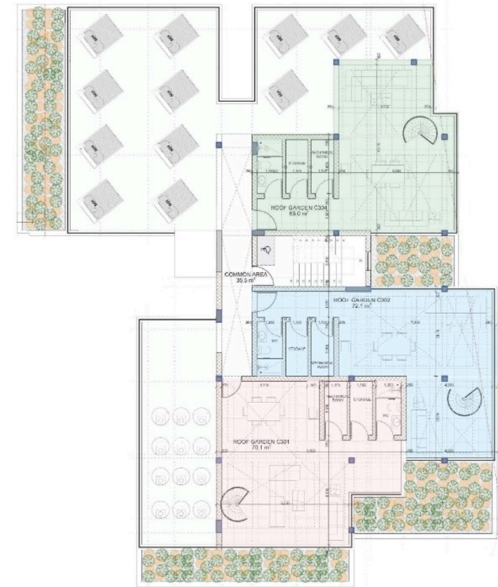
BLOCK C 4th FLOOR / ROOF GARDEN
