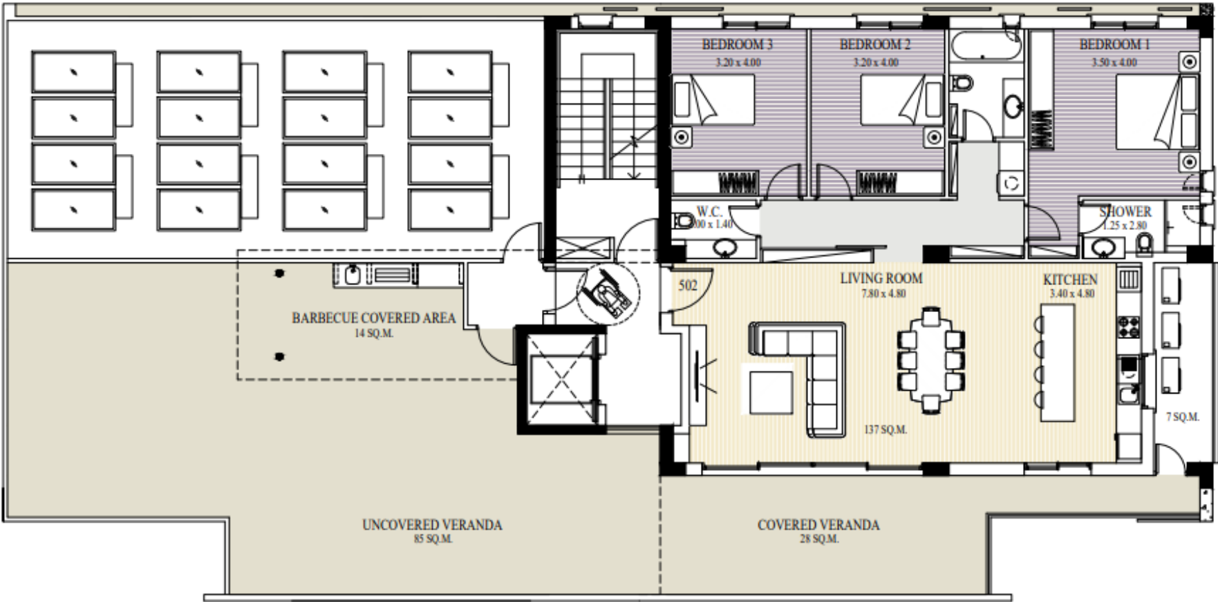
FIFTH FLOOR
