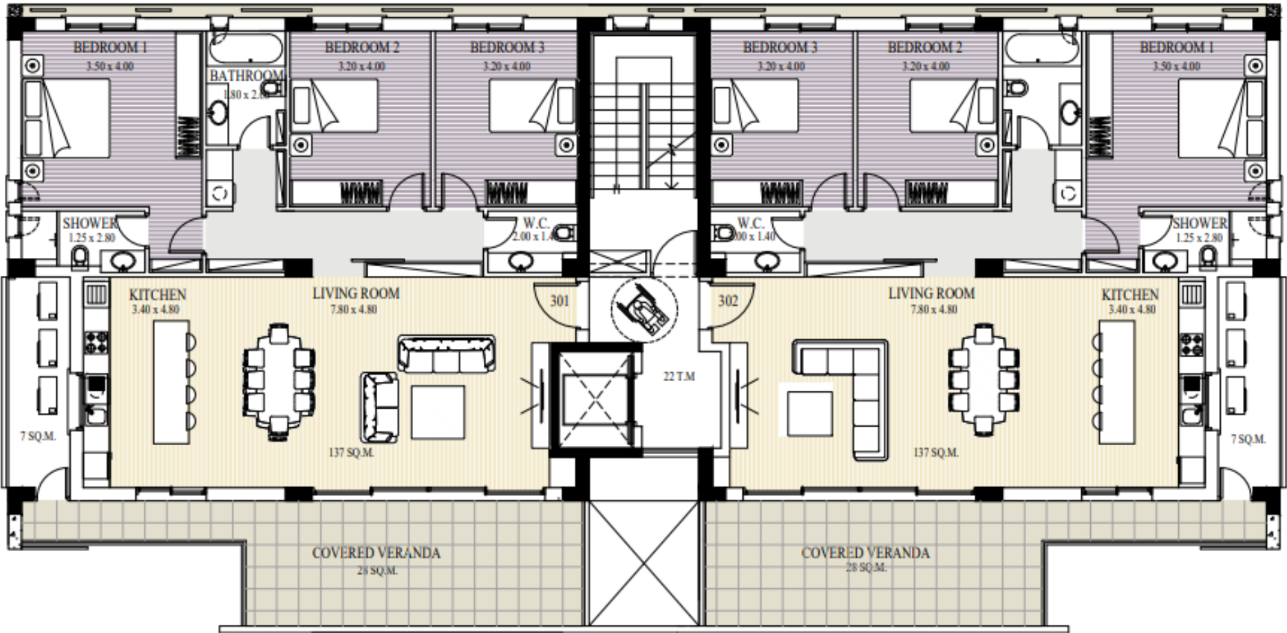
THIRD FLOOR
