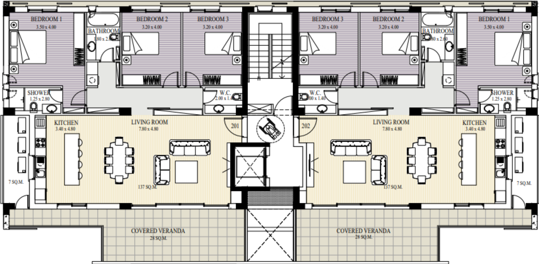
SECOND FLOOR
