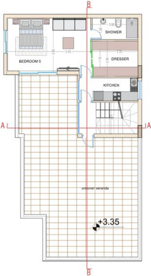
VILLA 1 - ROOF
