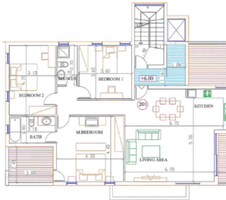
SECOND FLOOR PLANS APT 201
