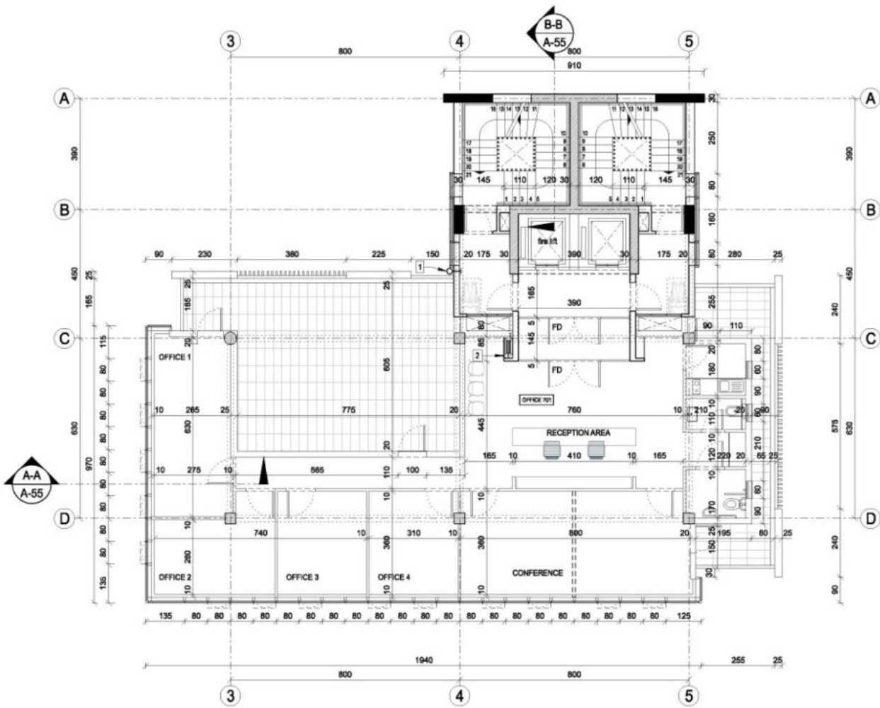
7th FLOOR PLAN
